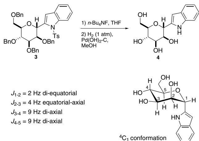
Scheme 1. Synthesis and conformation of \alpha -C-mannosylindole.
