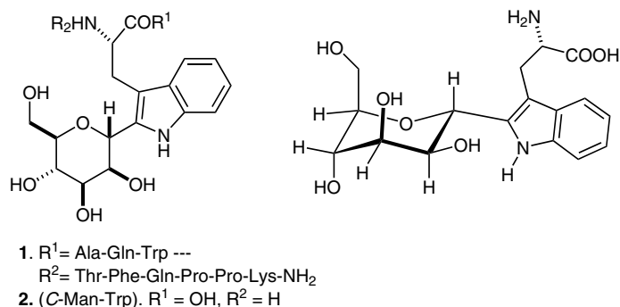
Figure 1. Chemical structure of \alpha - C -mannosyltryptophan.
