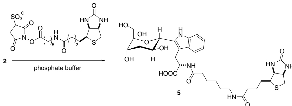
Scheme 2. Preparation of biotinyl C-Man-Trp.
