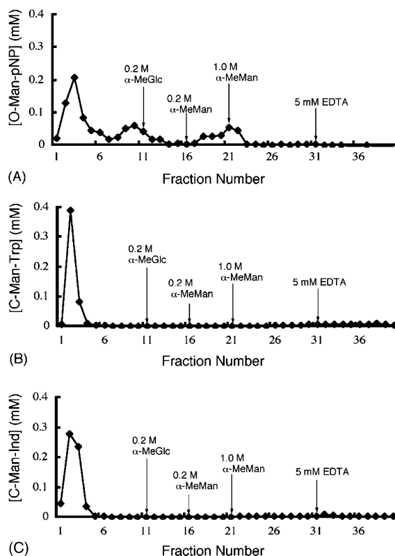
Figure 2. Affinity chromatograms on Con A-Sepharose column with O-Man-pNP (A), C -Man-Trp (B), and C -Man-Indole (C). (A) The concentration of O-Man-pNP was determined by measuring absorbance at 405 nm after hydrolysis of the mannoside. O-Man-pNP was retained in the column and eluted in fractions 18–22. O-Man-pNP was also eluted in the pass-through fractions because of overloading of the mannoside. (B) The concentration of C -Man-Trp was determined spectrophotometrically at 280 nm. In the pass-through fractions, 78% of the loaded C -Man-Trp were detected. C -Man-Trp was not found in any fractions eluted with \alpha -MeGlc, \alpha -MeMan or EDTA. (C) The concentration of C -Man-Indole was determined spectrophotometrically at 280 nm. In the pass-through fractions, 86% of the loaded C -Man-Indole were detected. C -Man-Indole was not found in any other fractions.
